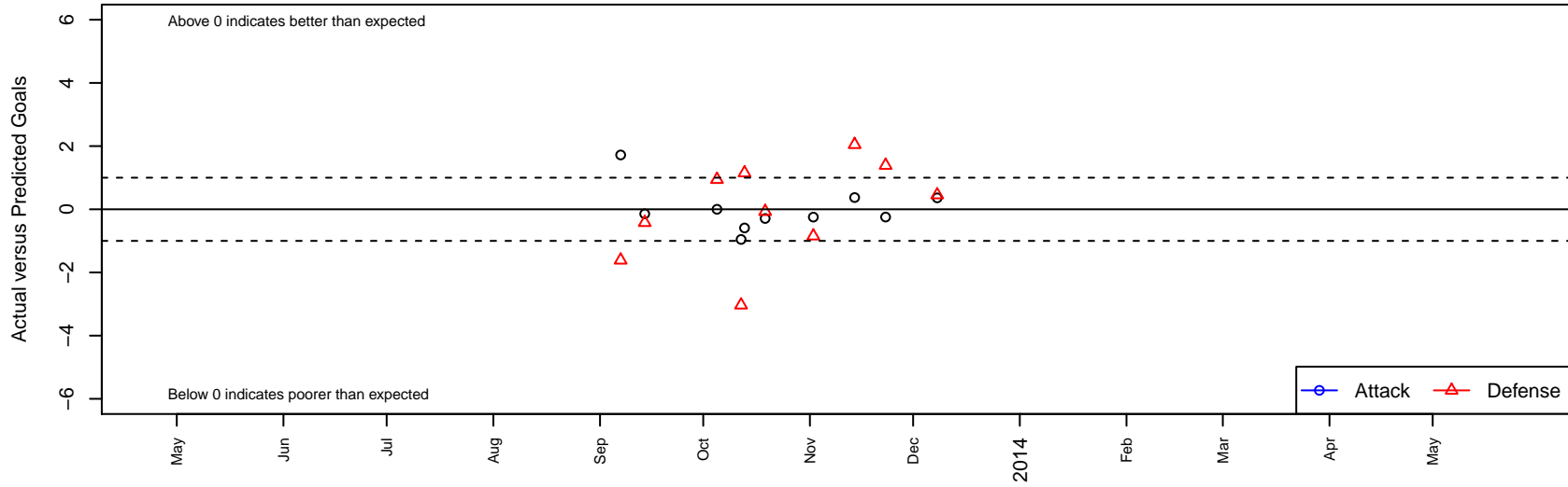
MFC United Red G00 Dots are actual minus expected GF (blue circles) and GA (red triangles). Blue line is smoothed change in attack strength. Red is smoothed change in defense strength.
